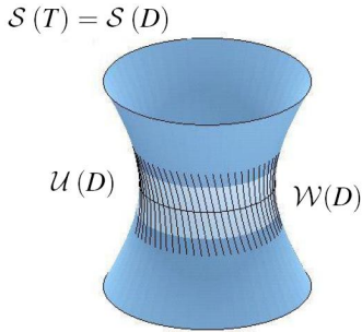
Figure 1: Union of stable manifolds
