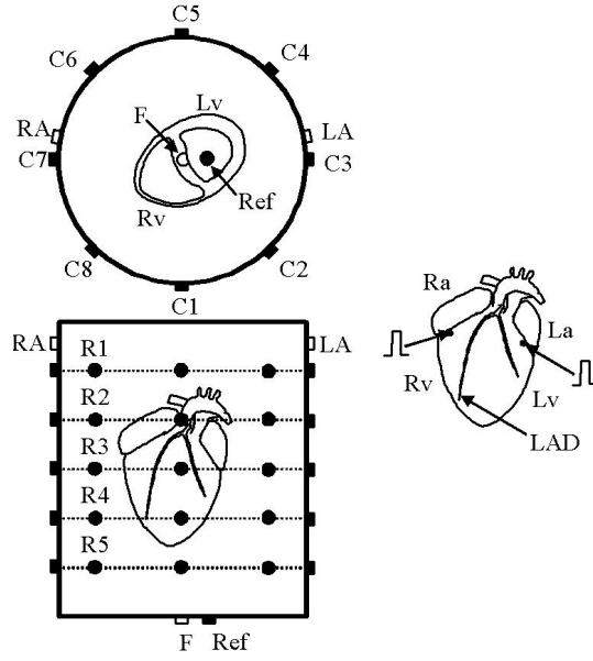
Figure 1: ECG multilead system: 40-electrodes configuration for electrocardiographic recording in the premature ventricular stimulation protocol. Schematic view showing the superior and frontal 5 \times 8 matrix electrodes, as well as the standard lead foot (F), left arm (LA), right arm (RA), and reference (Ref). Also are shown the positions of both the stimulating electrodes located in the base of the Lv and Rv, below the atrial appendages.
