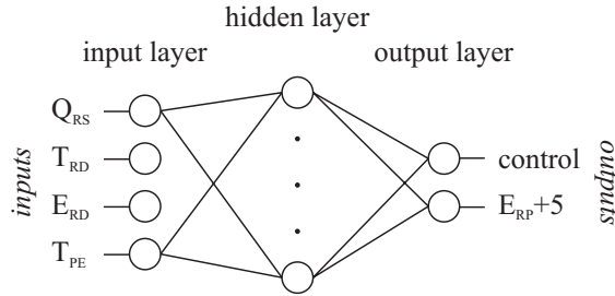
Figure 3: ANN topology with input and output signals used for classification of ECG data.
